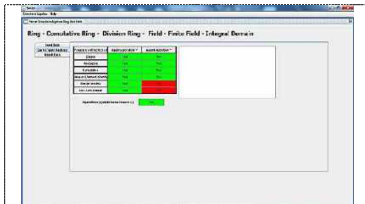
Figure 2. Cayley table analysis of set of matrices.
