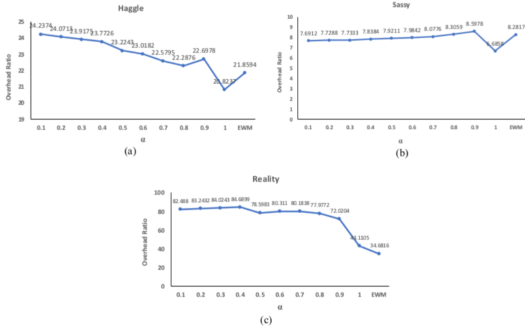
FIGURE 3. Overhead ratio of SimBet vs. SimBet-EWM in three different human mobility scenarios.
