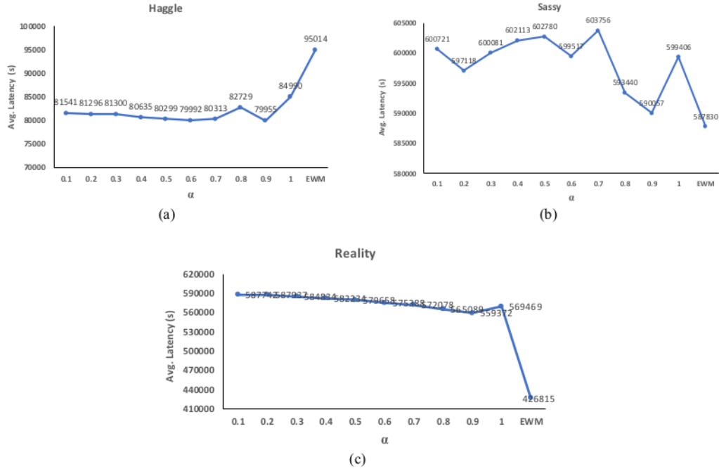
FIGURE 2. Delivery latency of SimBet vs. SimBet-EWM in three different human mobility scenarios.
