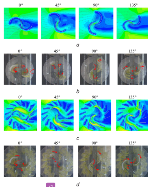
Fig. 5. Flow visualization: a – simulation results turbine without guide vanes, b – experiment results turbine without guide vanes, c – simulation results turbine with guide vanes, d – experiment results turbine with guide vanes
