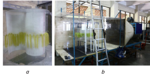
Fig. 4. Visualization Main signature: a – thread position on the blade; b – set up visualization
