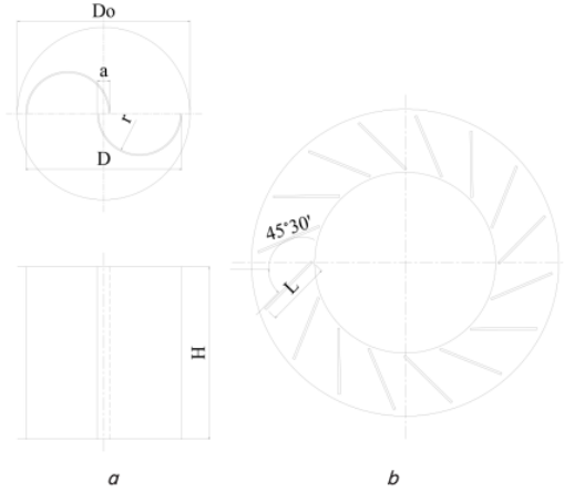
Fig. 2. Dimensions of Savonius wind turbine and guide vane Main signature: a – Sketch of the Savonius wind turbine, b – guide vane
