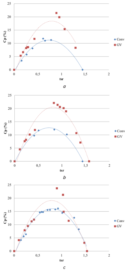
Fig. 8. Comparison of power factor of Conv and GV at the wind speed: a - 4 m/s; b - 5 m/s; c - 6 m/s
