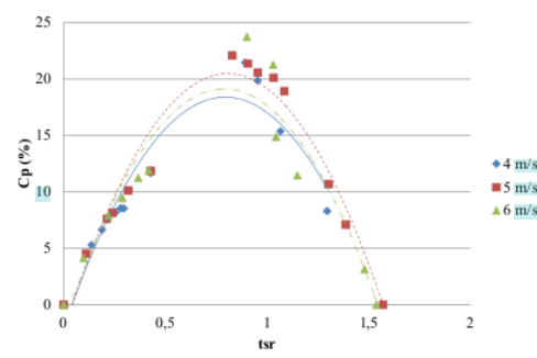
Fig. 9. Relationship between power factor and tsr on GV
