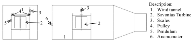
Fig. 3. Scheme of tools
