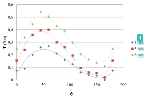
Fig. 7. Static torque to the wind speed at GV
