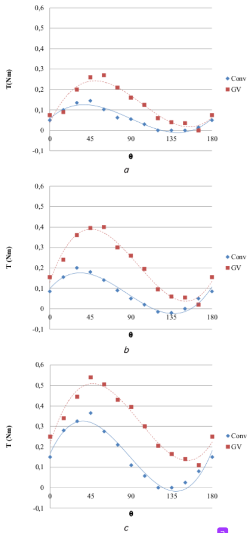
Fig. 6. Influence of guide vanes on static torque at speed: a - 4 m/s; b - 5 m/s; c - 6 m/s
