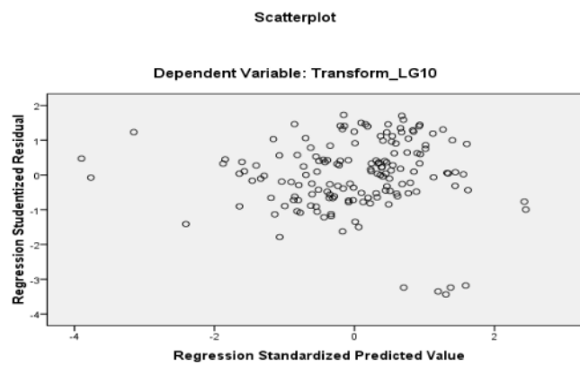
Figure 1. Heteroscedasticity Test Source: Processed data (2020)
