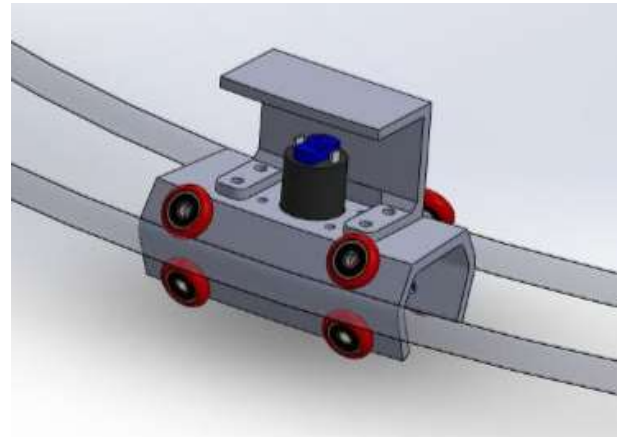
Figure 4. Camera Drive Mechanism
