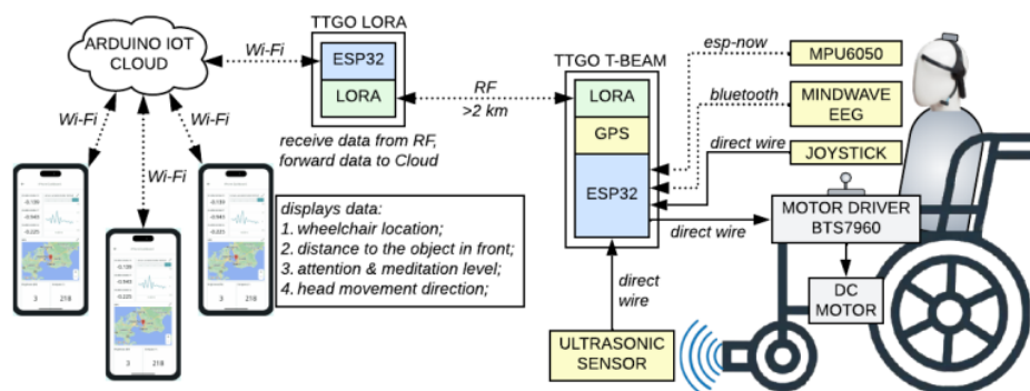
Figure 2. Block diagram of the wheelchair control system
