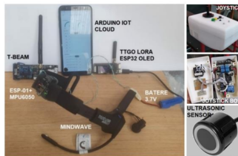
Figure 5. Components or devices used in the electric wheelchair control system, including Arduino IoT cloud
