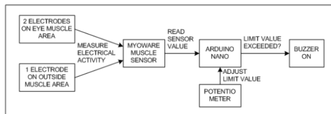
Fig 5: Function Block Diagram of Drowsiness Alert System
