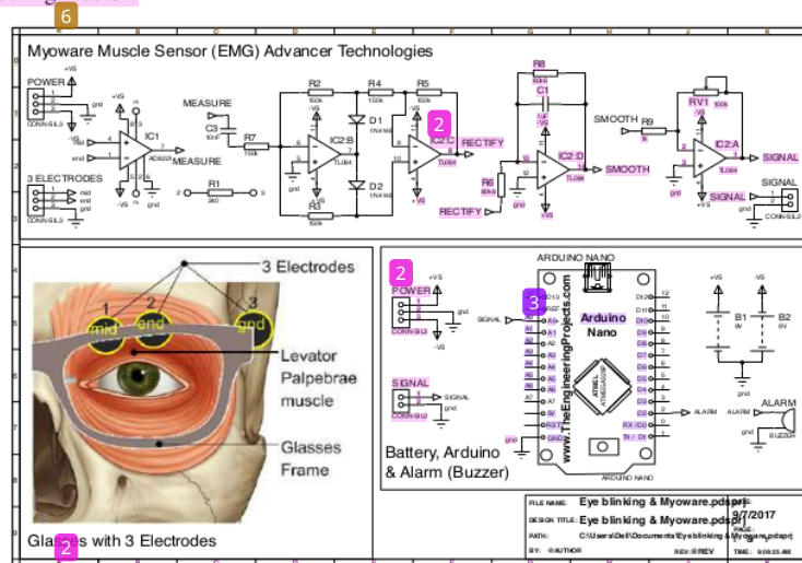
Fig. 2: Circuit Schematic and electrodes placement on eyeglass
