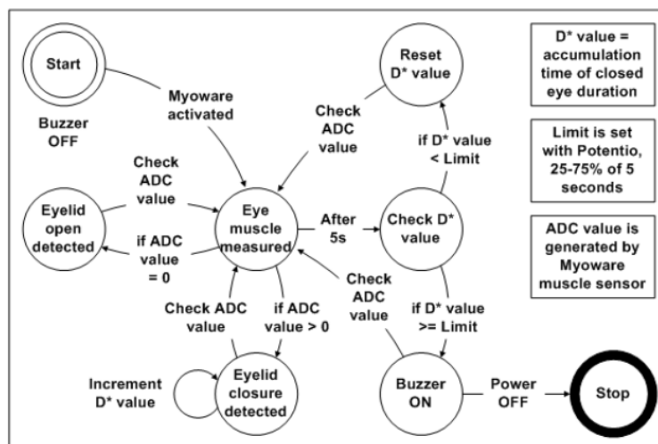
Fig 6: State Diagram of Drowsiness Alert System
