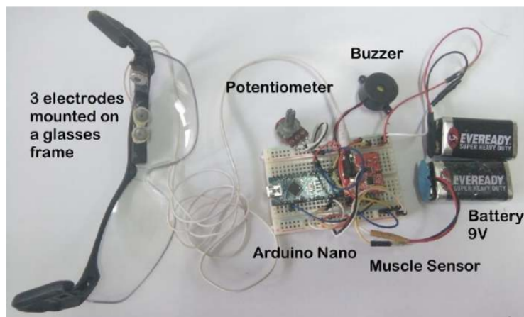
Fig. 1: The hardware prototype of drowsiness detection device
