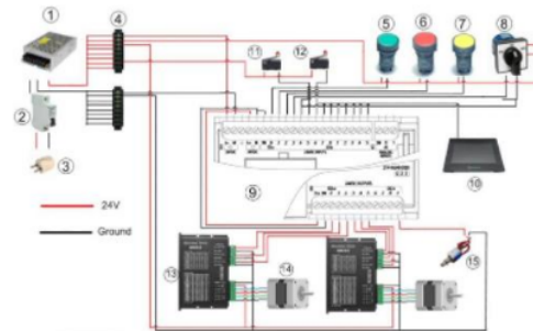
Figure 4. Electrical circuit
