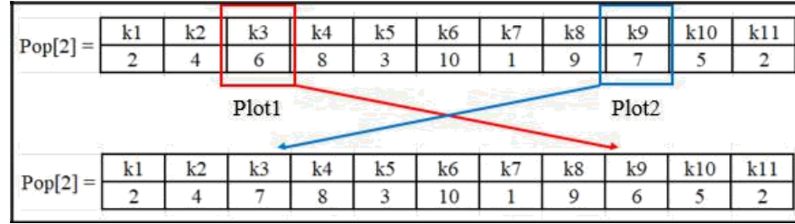
Fig 4. Reciprocal Mutation
