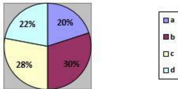
Fig 2. Roulette Wheel
