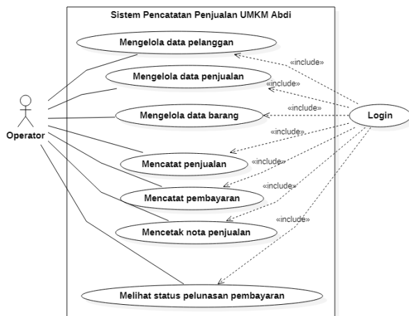
Gambar 3. Diagram Use-Case
