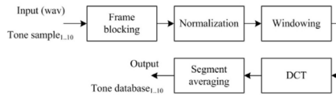
Figure-4. Block diagram of the tone database generation.
