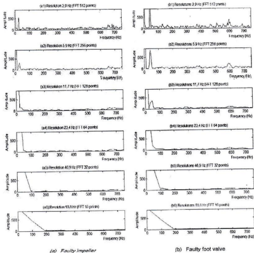
Figure 9. Graphical displays of water pump vibrations in the frequency domain on X axis direction, for a faulty impeller and a faulty foot valve bearing water pumps
