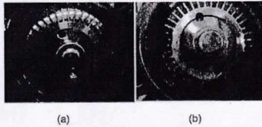
Figure 3. Impeller examples; (a) A good impeller; (b) A faulty impeller due to wear
