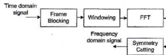
Figure 6. Block diagram of the conversion steps [9]
