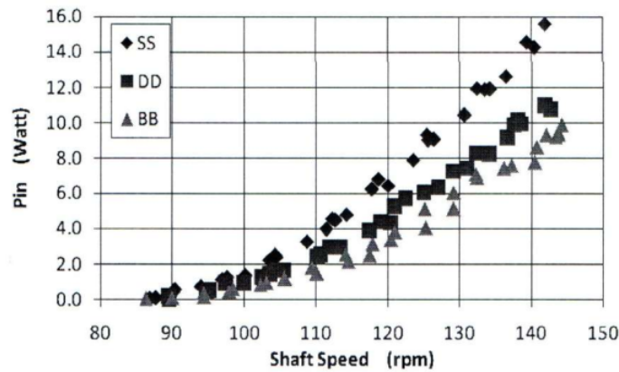
Figure 6. Shaft power inputs and shaft speed
