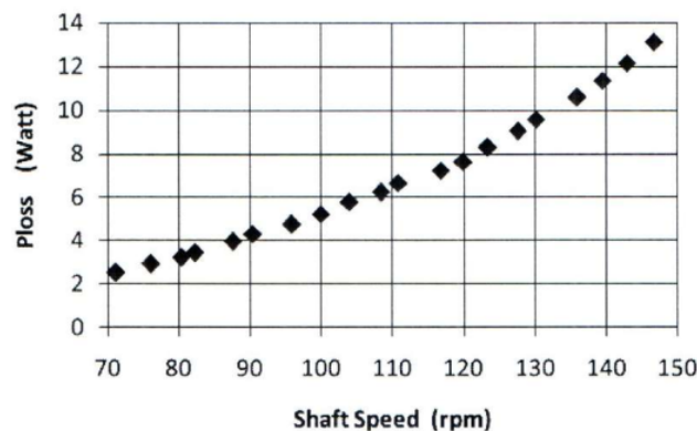
Figure 4. Mechanical power losses and shaft speed
