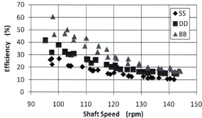
Figure 7. Pumps efficiencies and shaft speed
