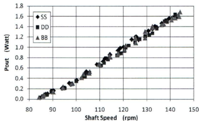
Figure 5. Pumping power outputs and shaft speed
