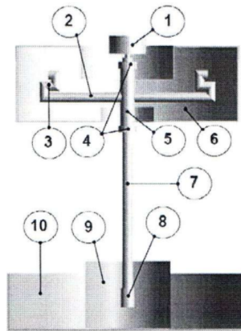
Figure 1. Schematic of centrifugal reaction pump.
