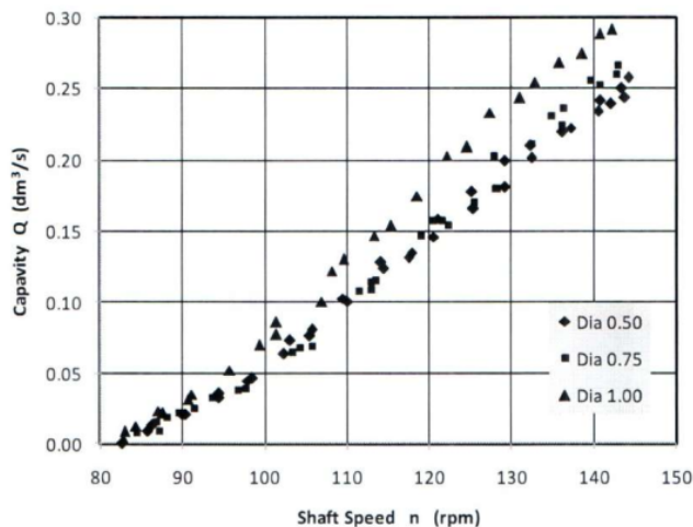
Figure 8. Pumps capacity and shaft speed
