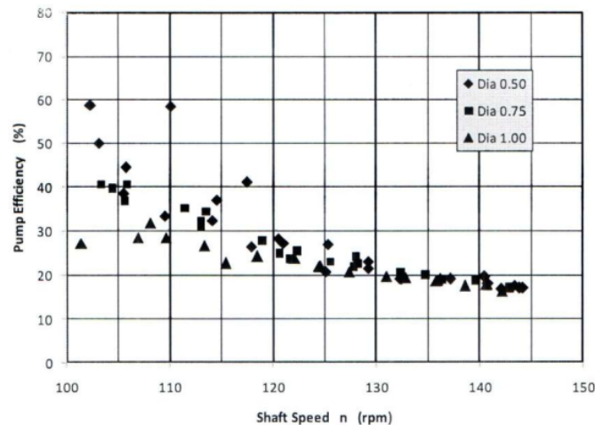
Figure 9. Pumps efficiency and shaft speed
