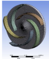
Gambar 2. Solid Mesh
