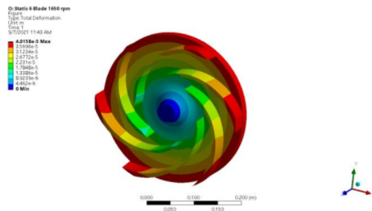
Gambar 11. Contour Total Deformasi Impeller
