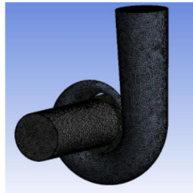
Gambar 1. Fluid Mesh
