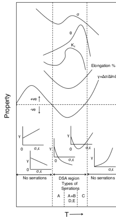
Gambar 1: Penentuan area serrated yielding berdasarkan sifat mekanis [10].
