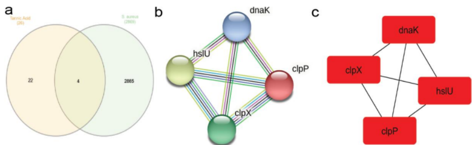
Figure 2. Bioinformatics Analysis of Staphylococcus aureus protein interacting with tannic acid a. Venn Diagram showing interacting protein of S.aureus to tannic acid. b. Protein-protein interaction network of tannic acid and the interacting proteins. Top 4 rank of S.aureus gen interacting to tannic acid based on MCC (Maximal Clique Centrality).
