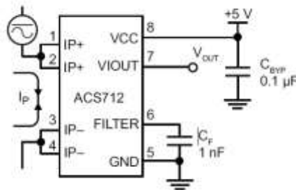
Gambar 3. Rangkaian sensor arus ACS712-30A (Allegro, 2013).
