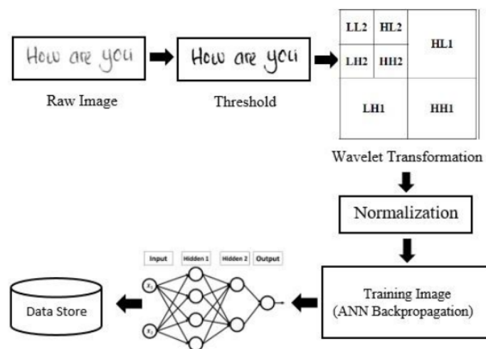
Figure 4. Training Phase
