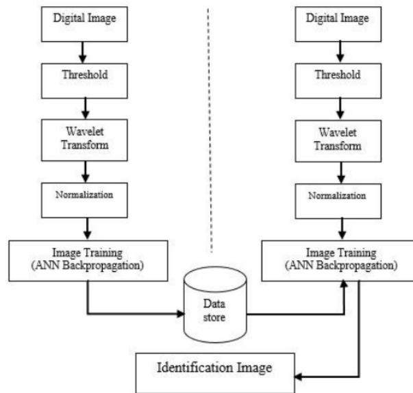
Figure 3. Handwriting Identification Flowchart
