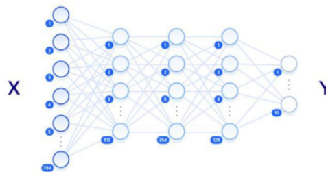
Figure 1. Artificial Neural Network Architecture [4]
