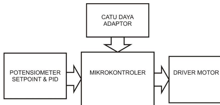
Gambar 1. Diagram blok piranti pengendali PID
