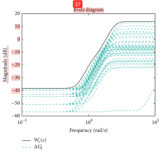
FIGURE 16: Complementary sensitivity weight W_t(s) and the system uncertainty of the hip joint control.
