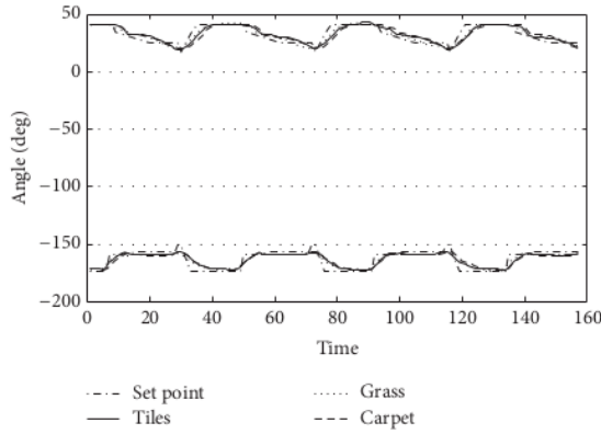
FIGURE 30: Gait trajectory tracking performance when trotting on three different surfaces: hard tiles, grass, and carpet.
