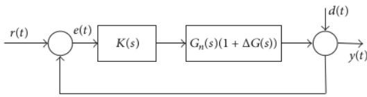
FIGURE 11: Single-input single-output controlled system with perturbation.
