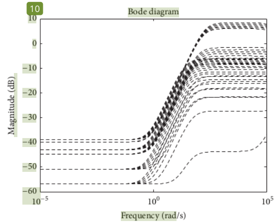
FIGURE 13: Model uncertainty of knee motor and its load singular plots.
