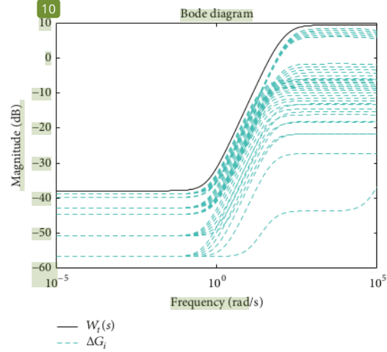
FIGURE 17: Complementary sensitivity weight W_t(s) and the system uncertainty of the knee joint control.
