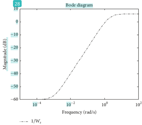
FIGURE 15: Inverse of sensitivity weight W_s(s) .
