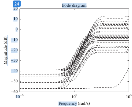
FIGURE 12: Model uncertainty of hip motor and its load singular plots.
