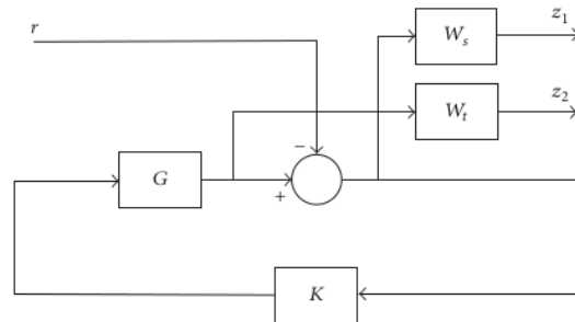
FIGURE 14: Mixed sensitivity control block diagram.
