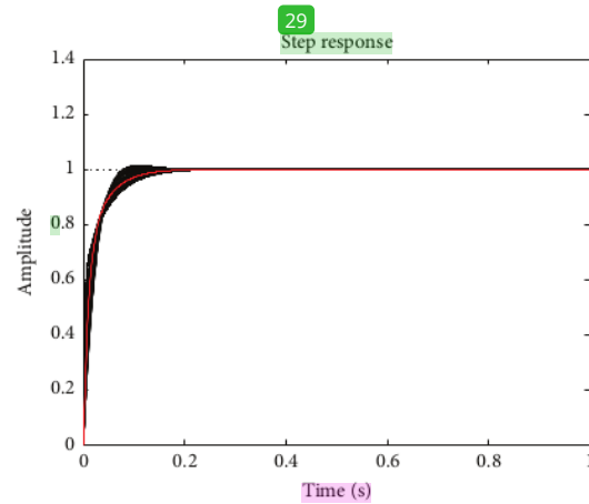
FIGURE 25: Simulation result of the proposed controller on the knee joint under uncertainty.
