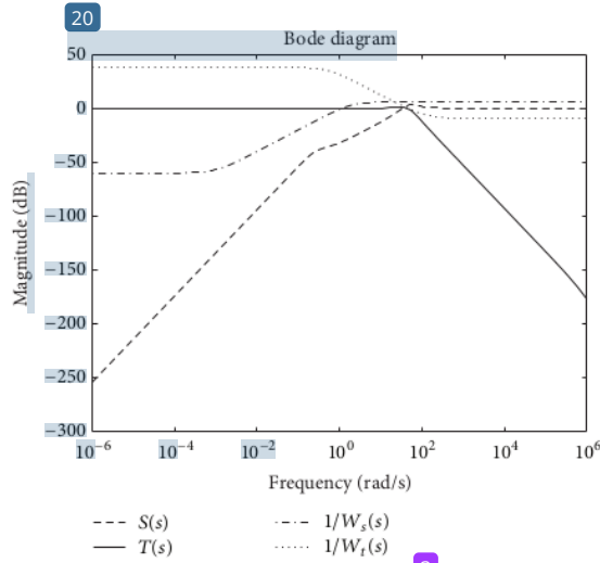
FIGURE 19: The sensitivity, complementary sensitivity, and their inverse of the weight singular values of the knee joint.
