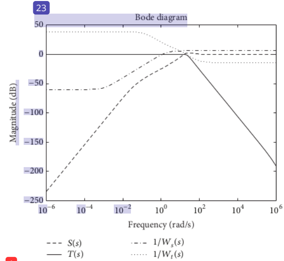
FIGURE 18: The sensitivity, complementary sensitivity, and their inverse of the weight singular values of the hip joint.
