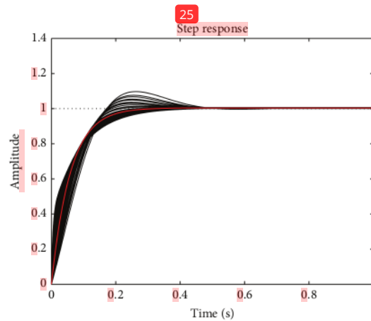
FIGURE 22: Simulation result of the controller on the hip.
