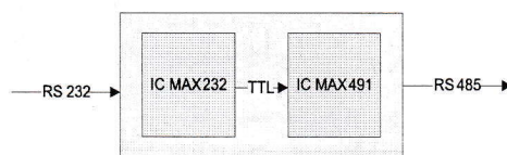
Gambar 8. Konverter RS232-RS485
