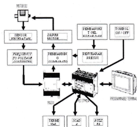
Gambar 5. Diagram blok perancangan plant 1 terkoneksi PLC 1 (Cahyono, E., 2009)
