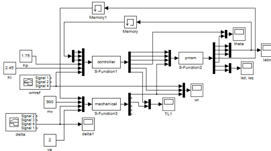
Fig. 5. The implementation of the electric vehicle in Simulink/Matlab
