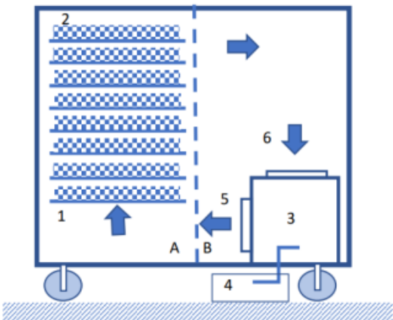
Fig. 4. The oven and the equipment setup.
