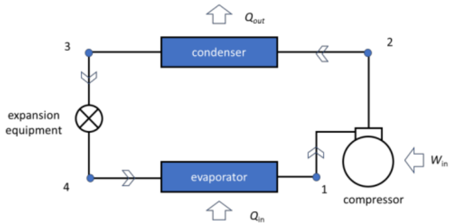
Fig. 2. The Refrigerator sections.
