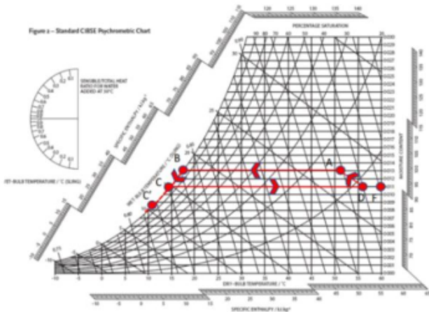
Fig. 6. c. The air cycle at 55 hours drying
