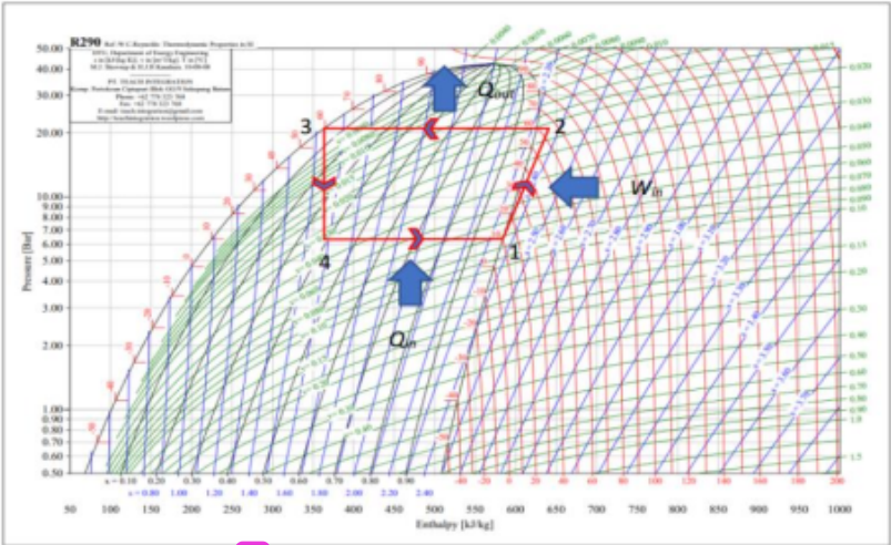
2 Fig. 7. The vapor compression cycle of R-290.
