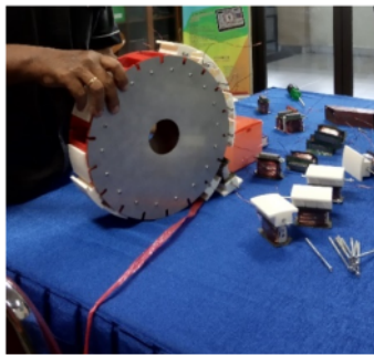
FIGURE 2. Coils on the shell and the stator frame where the coils are placed.
