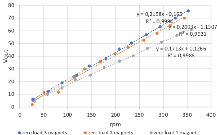
FIGURE 4. The output voltage as the function of the rotation speed in condition without load.
