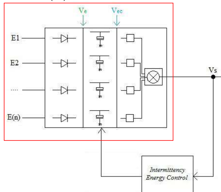
Gambar 4. Blok Diagram Multiplexing and Summing Power
