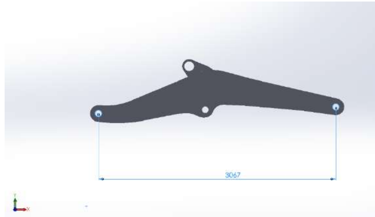
Gambar 3. Lift arm awal
