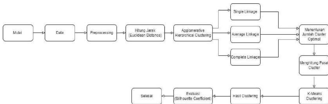
Gambar 1 Diagram Alur Kerja Hierarchical K-Means Clustering
