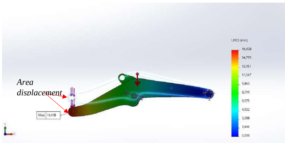
Gambar 9. Distribusi displacement posisi 1
