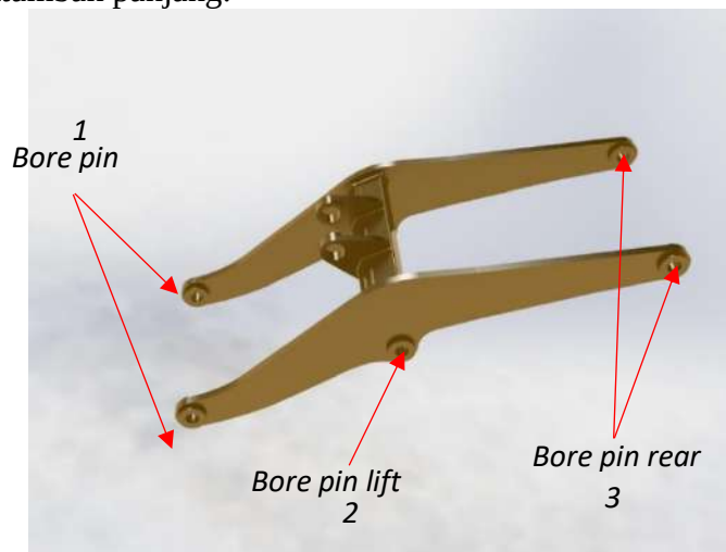
Gambar 2. Hasil rendering desain lift arm WA470
