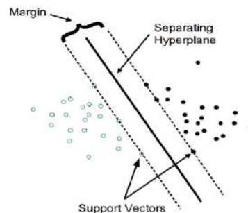
Gambar 2. Support Vector Machine
