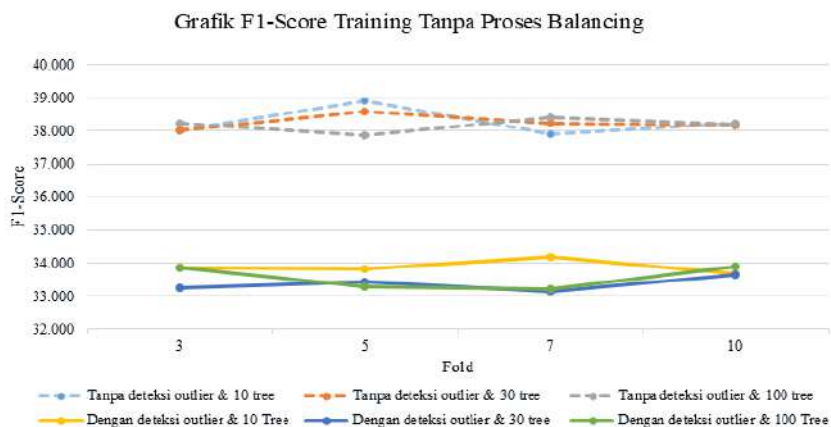
Gambar 13. Grafik hasil f1-score training tanpa proses balancing
