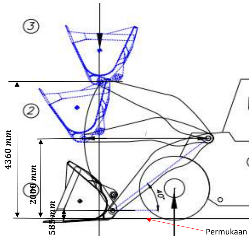
Gambar 1. Variasi Penelitian lift arm loader WA470
